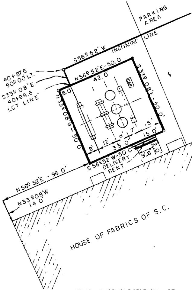
DETAILS OF SUBSTATION LOT SCALE 1" = 30'
