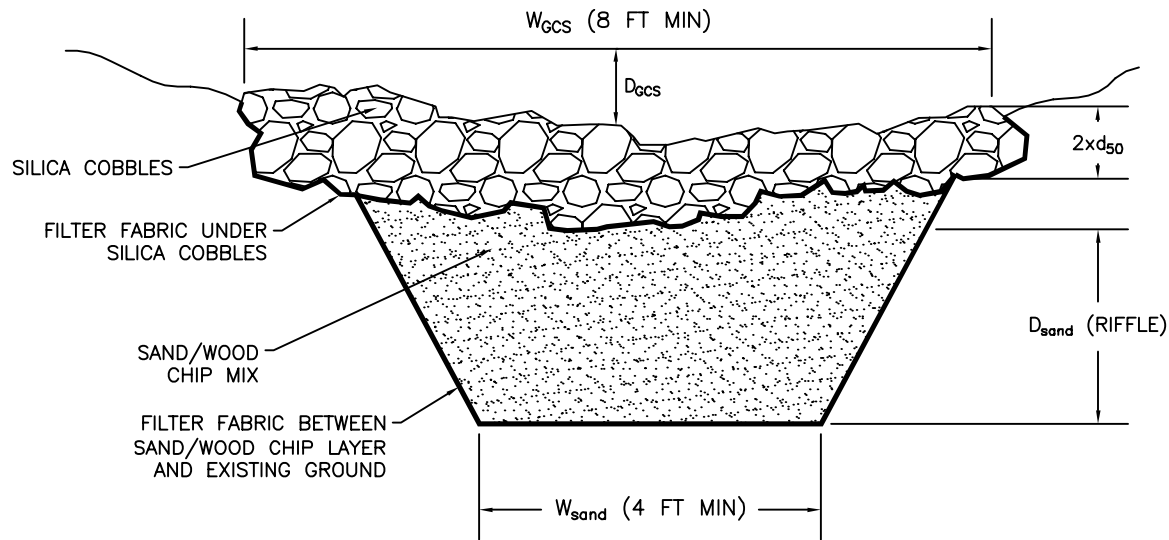
SECTION A-A' RIFFLE WEIR GRADE CONTROL STRUCTURE CROSS SECTION
