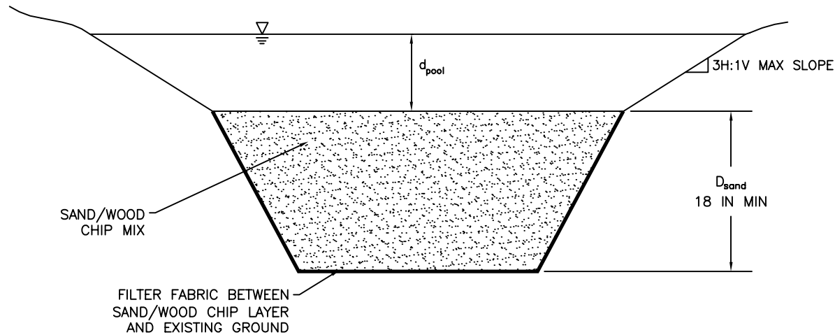
SECTION B-B' POOL CROSS SECTION
