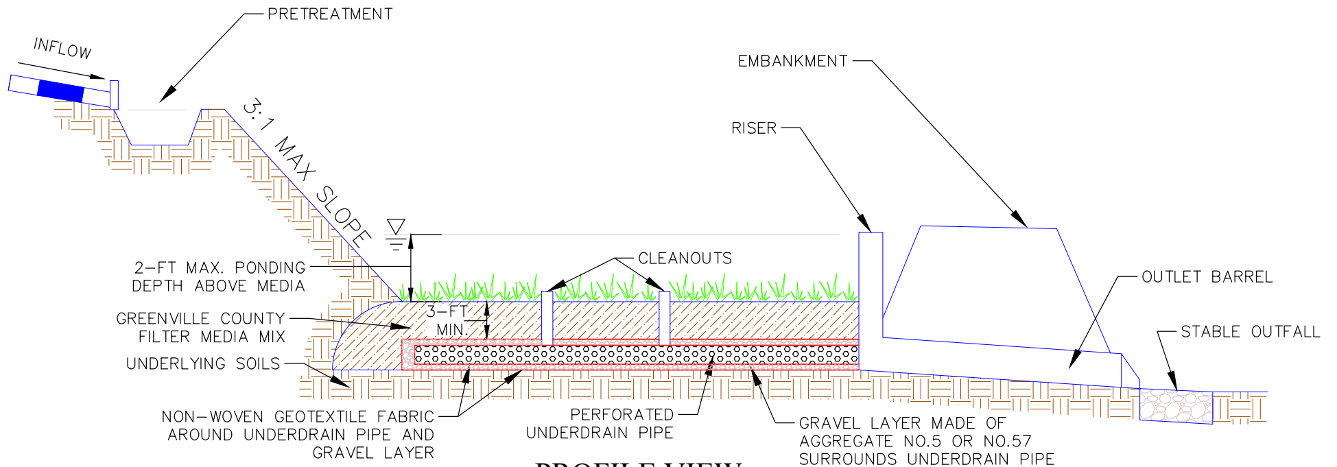
PROFILE VIEW
