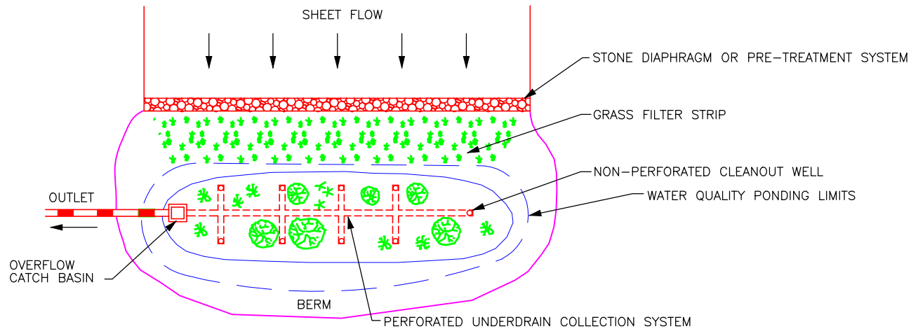
PLAN VIEW
