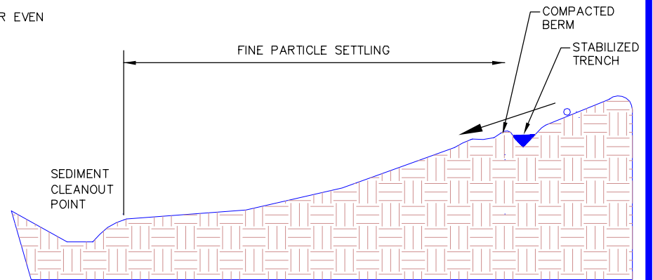
PROFILE VIEW
