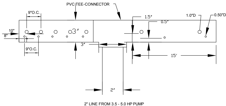
OUTLET STRUCTURE TO VEGETATED BUFFER
