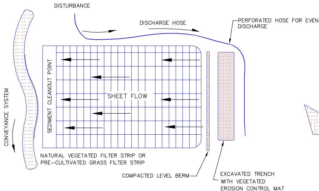
PLAN VIEW
