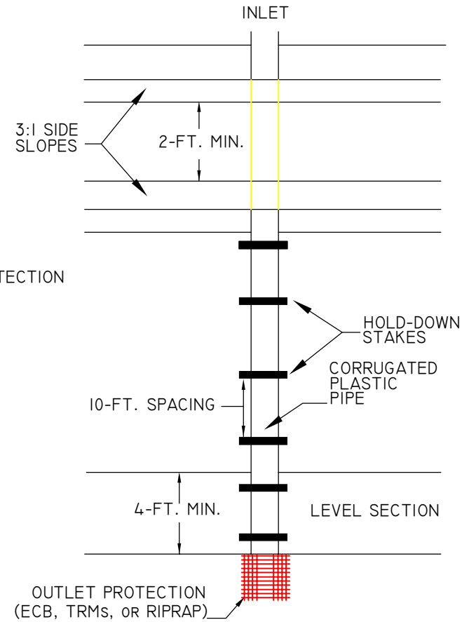
PLAN VIEW
