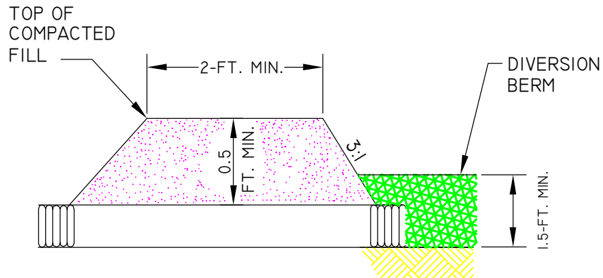
LEVEL SECTION
