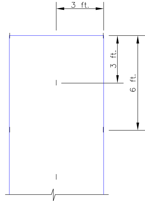
ANCHOR PATTERN FOR SLOPES FLATTER THAN 3:1
