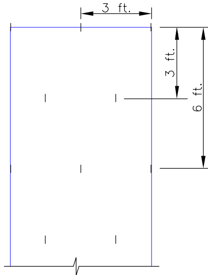
ANCHOR PATTERN FOR SLOPES BETWEEN 3:1 AND 2:1
