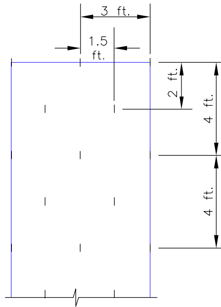
ANCHOR PATTERN FOR SLOPES BETWEEN 2:1 AND 1:1
