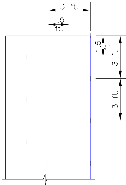
ANCHOR PATTERN FOR SLOPES GREATER THAN 1:1
