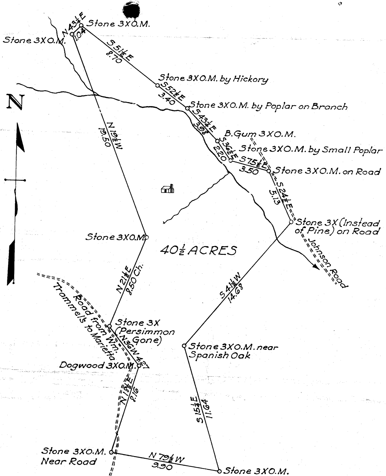
PLAT OF 40 1/2 ACRES MISS MARY E. BATSON (This Tracing Made Nov., 1935 from Survey Made by Mr. Will D. Neves, Surveyor, Feb. 26, 1903)
