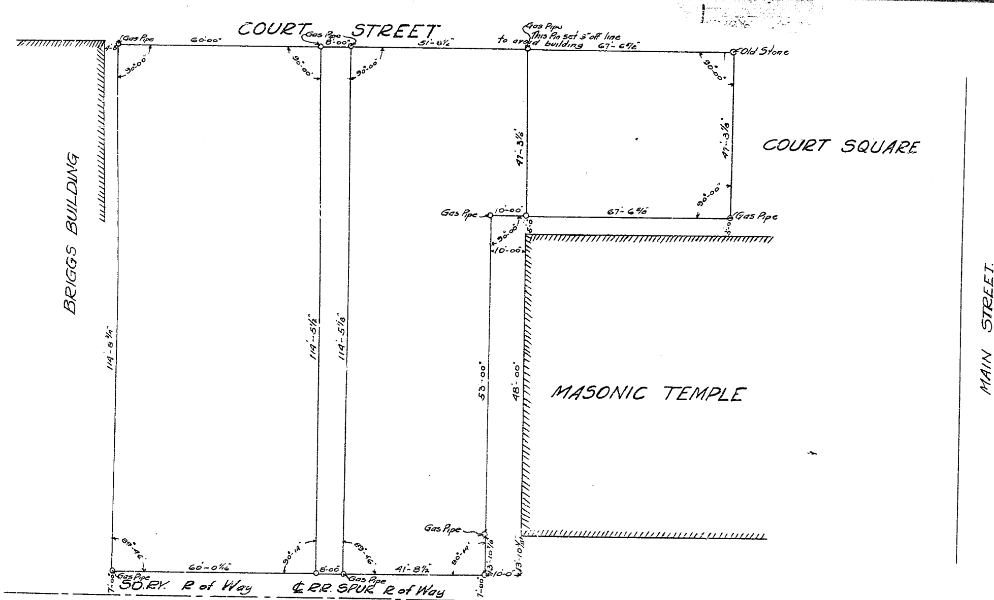
PLAT OF DONALDSON PROPERTY. COURT ST. & COURT SQUARE GREENVILLE S.C. SCALE 1/4" = 20 FEET. SURVEYED BY WGP.
