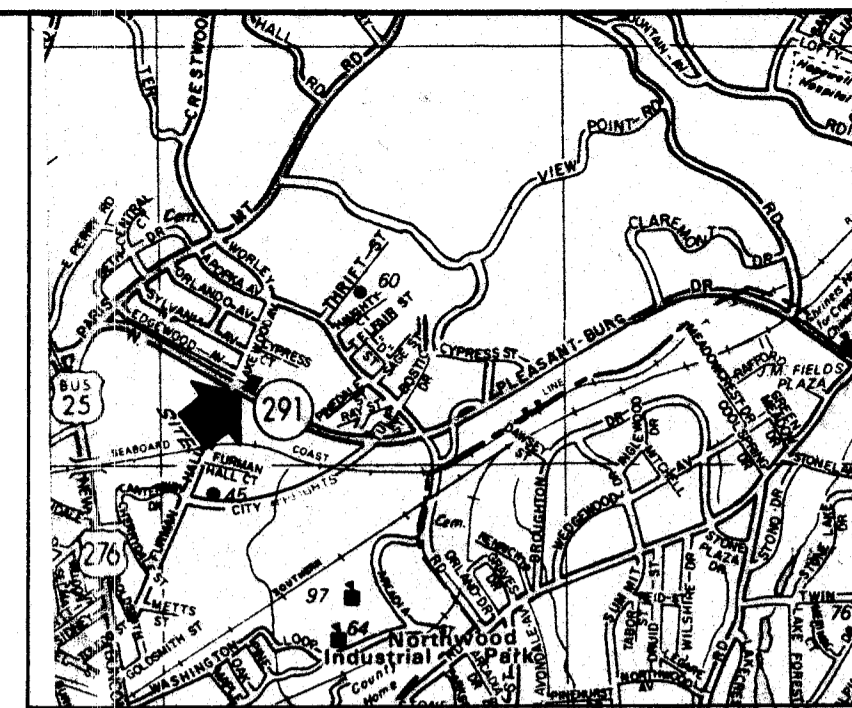
LOCATION MAP
