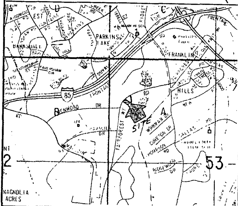
LOCATION MAP
