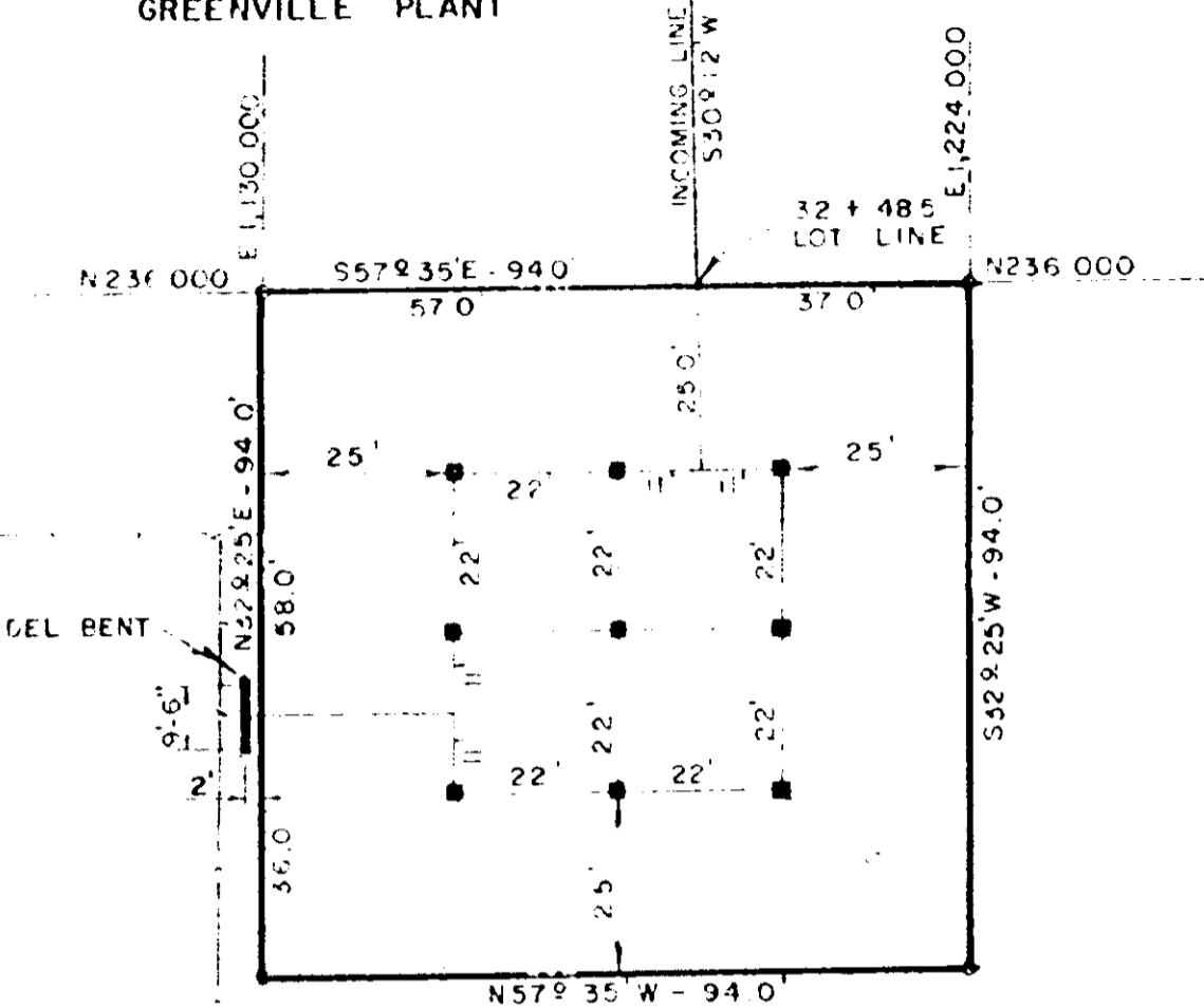
DETAILS OF SUBSTATION LOT #2
