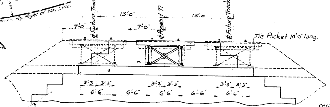
Slope 1 1/2 to 1 Square to track Section through bridge Scale 1/8" = 1'-0"
