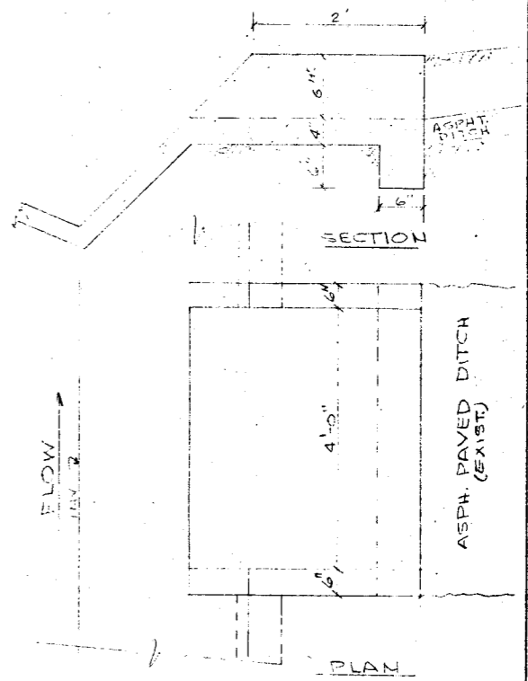
DETAIL OF TIE-IN OF ASPH. PAVED DITCH TO CONCRETE PAVED DITCH. N/S
