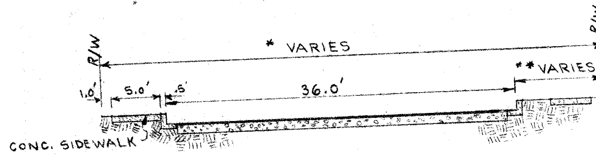
SECTION A-A STREET DETAIL
