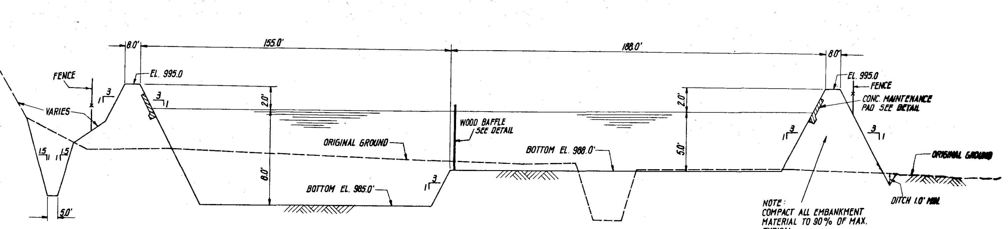
TYPICAL SECTION THRU TREATMENT FACILITY "A-A" SCALE: 1" = 30' HOR. 1" = 5' VERT.
