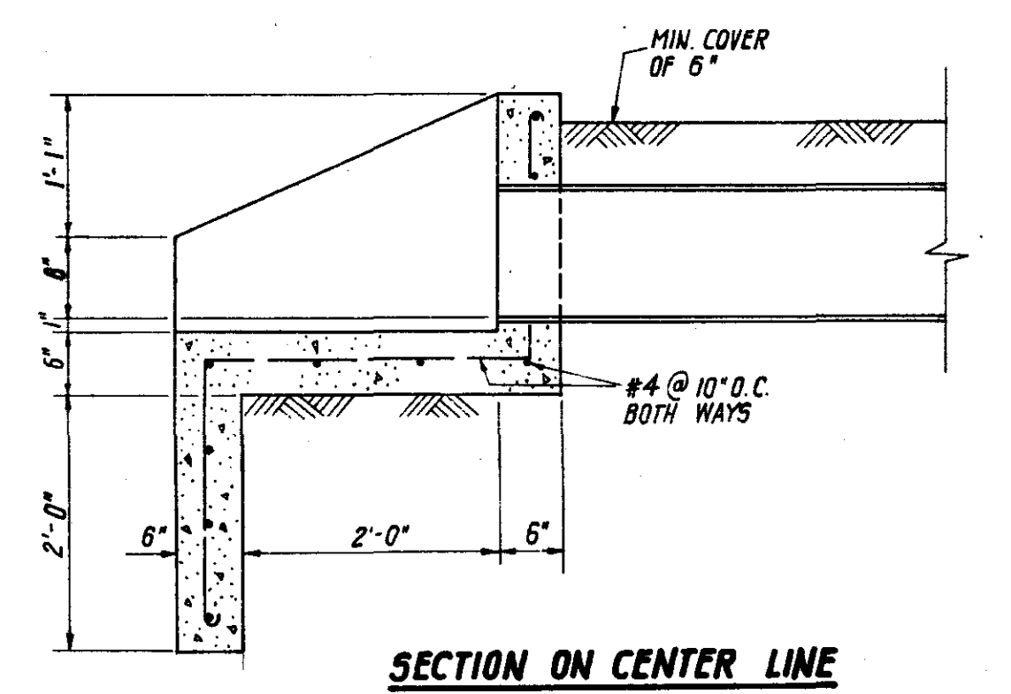
HEADWALL DETAIL AT EFFLUENT DISCHARGE
