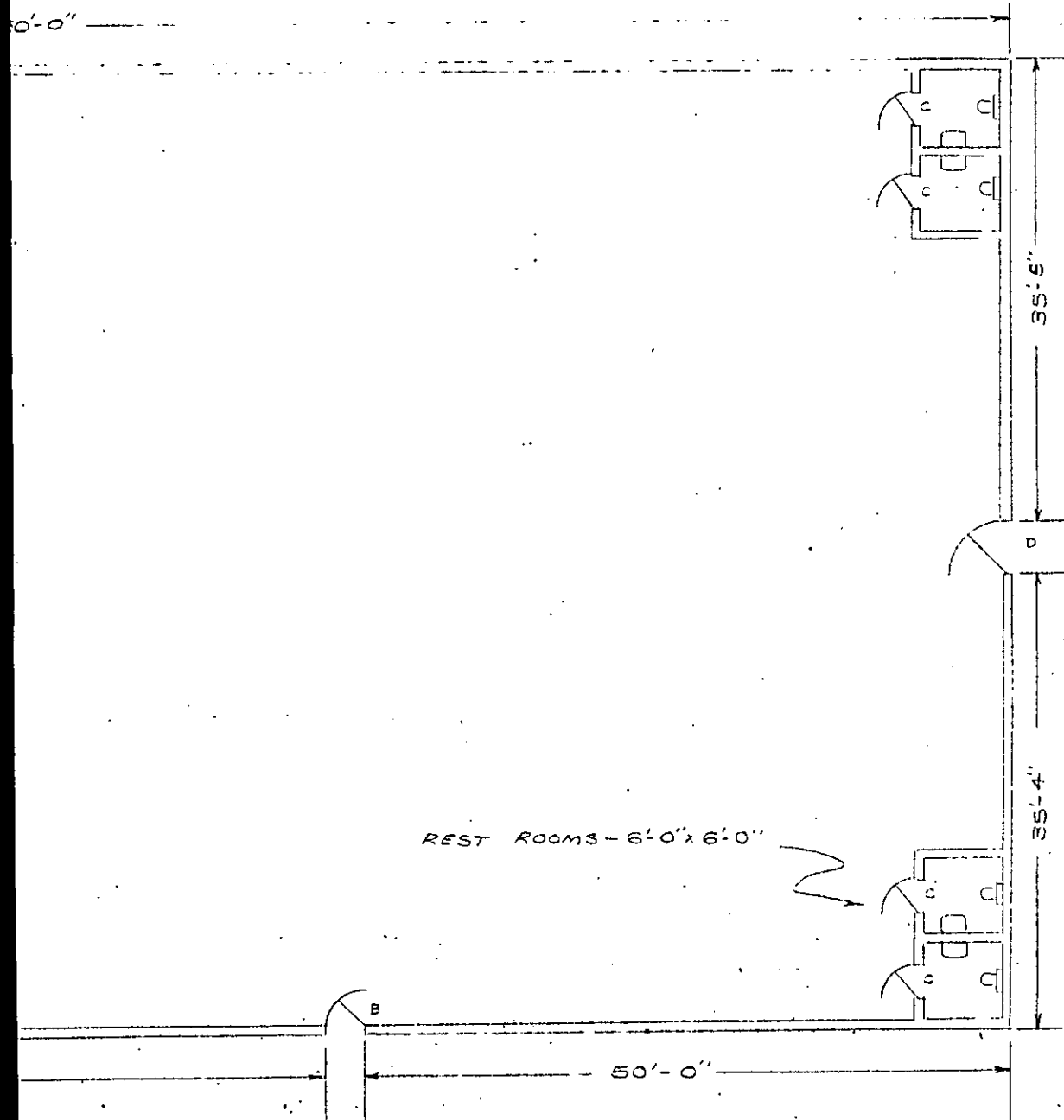
PLAN 3/32" = 1'-0"
