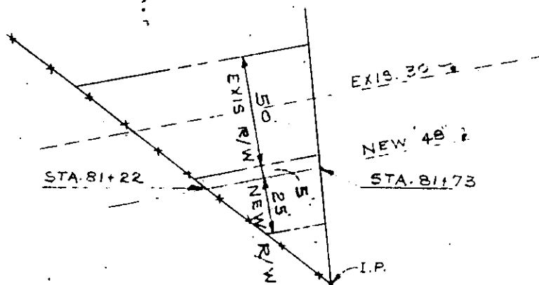
PLAN DETAIL SCALE 1" = 50'
