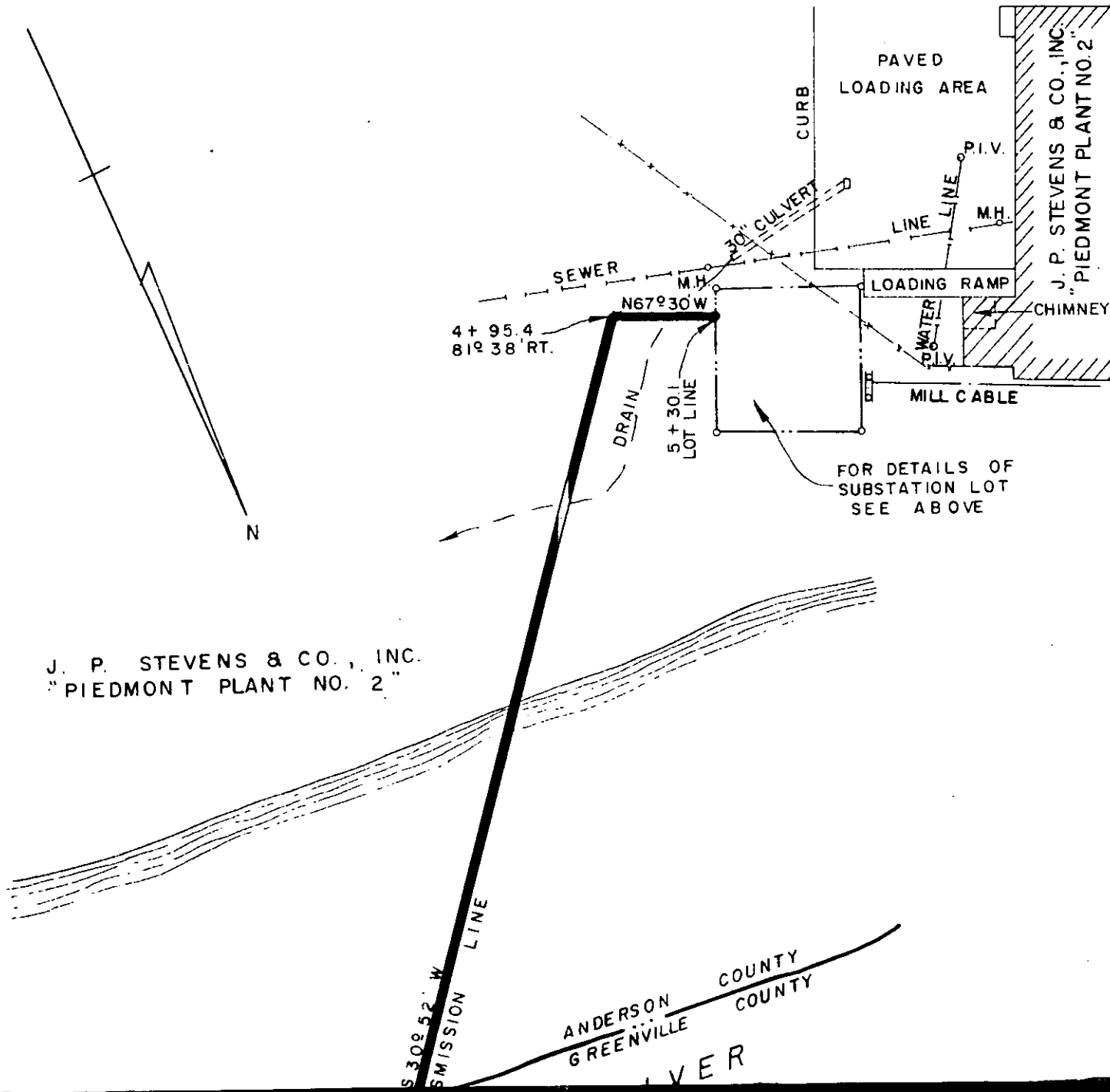
DETAILS OF SUBSTATION LOT SCALE: 1" = 30'
