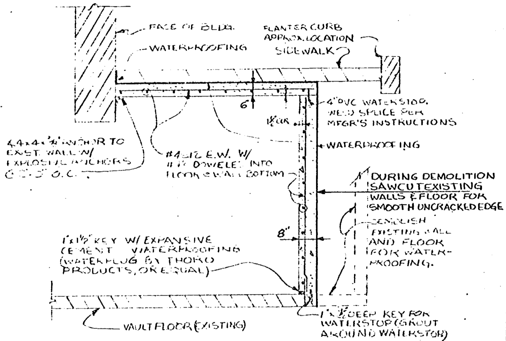
SECTION T-T SCALE 1/2" = 1'-0"
