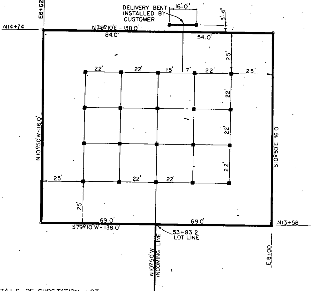
DETAILS OF SUBSTATION LOT SCALE: 1" = 30'
