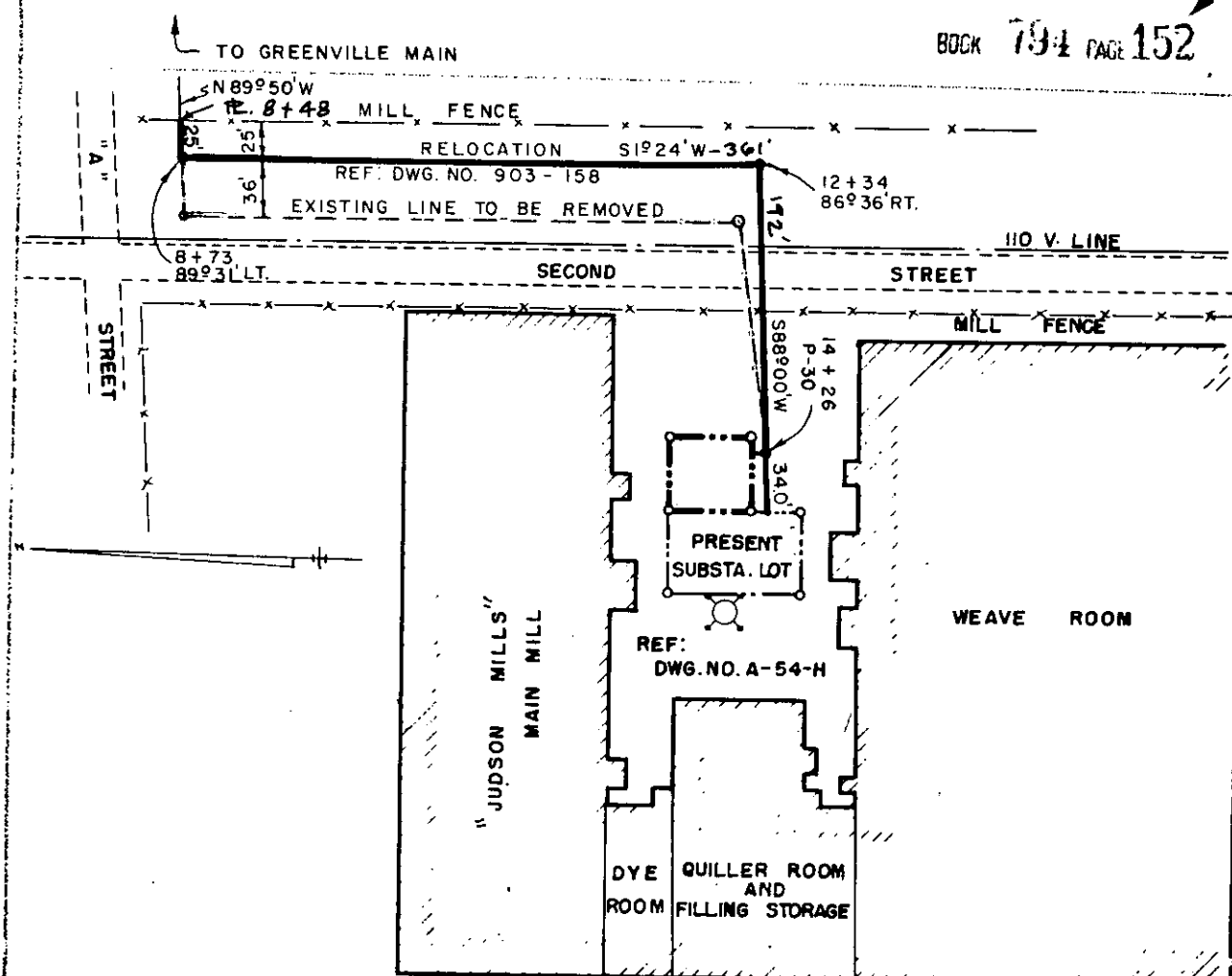
ALIGNMENT OF LINE SCALE: 1"=100'
