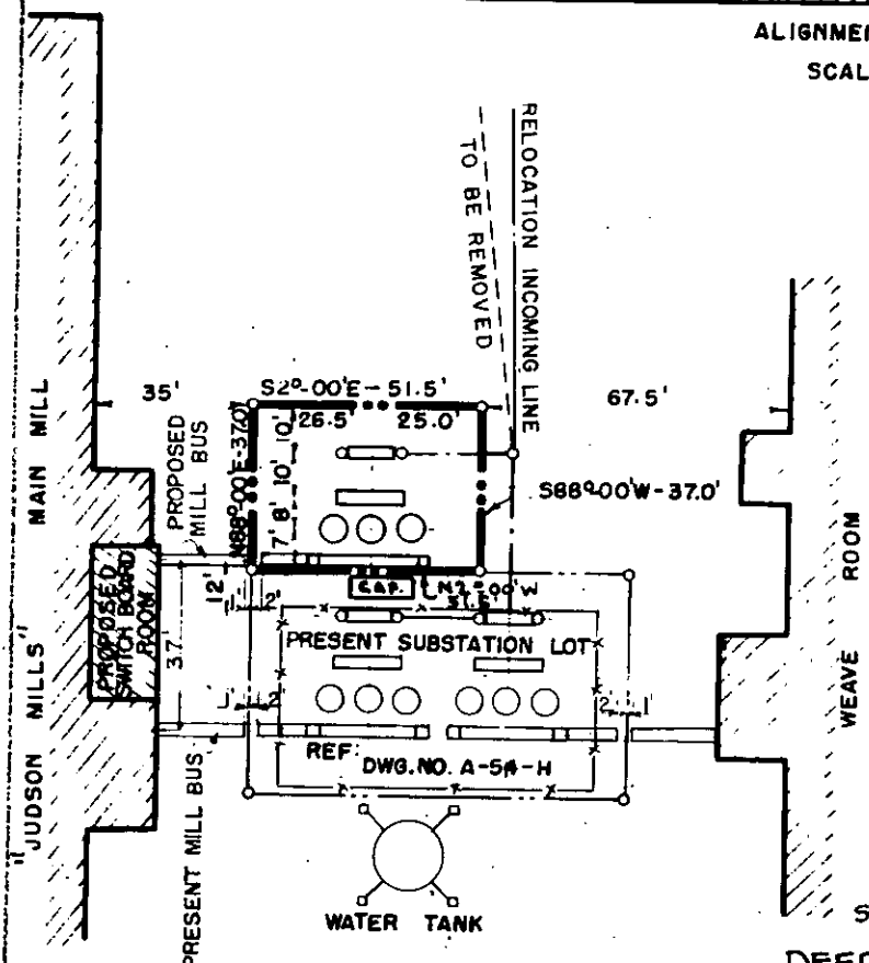
DETAILS OF SUBSTATION LOT SCALE: 1"=40'
