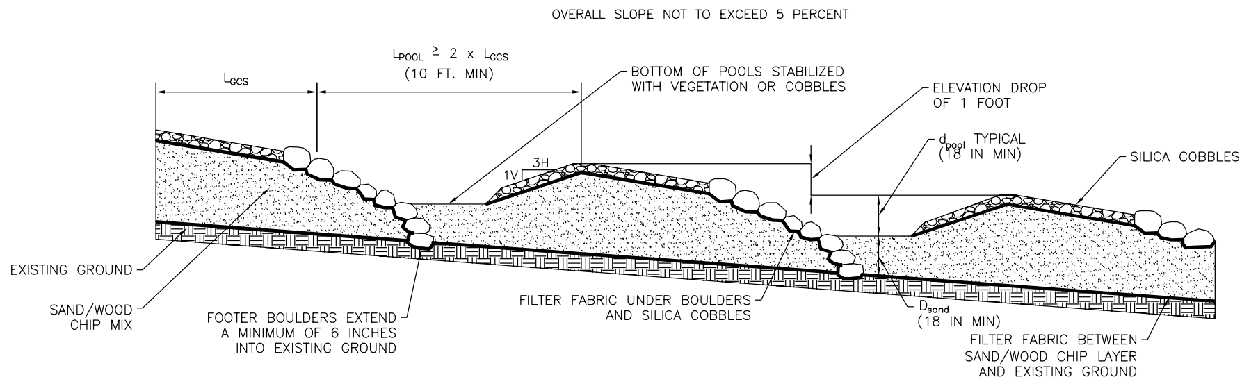
TYPICAL PROFILE - ALTERNATING POOLS AND RIFFLES
