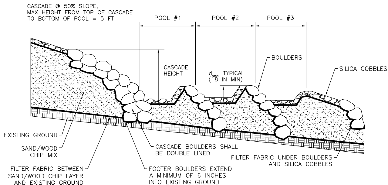
CASCADE PROFILE - THREE POOLS FOLLOWING CASCADE
