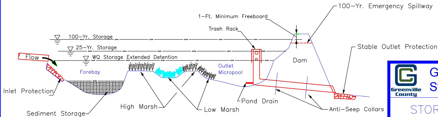
PLAN VIEW
