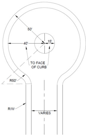
STANDARD TURNING AREA (C)
