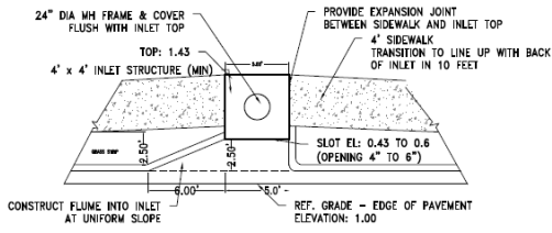
TYPE 9 INLET (RUN LOCATION) NOT TO SCALE
