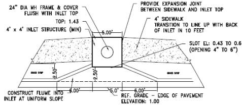
TYPE 9 INLET (SAG LOCATION) NOT TO SCALE
