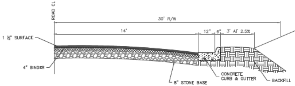
INDUSTRIAL/COMMERCIAL STANDARD
