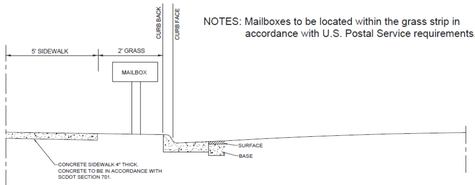
Exhibit 8.5 Typical Mailbox and Sidewalk Location
