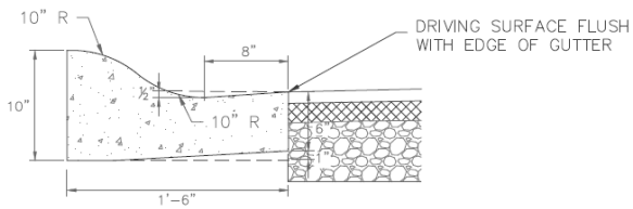
ROLLED CURBING
