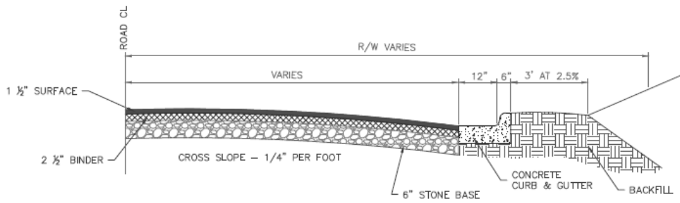
URBAN STANDARD
