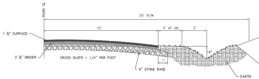
RURAL STANDARD
