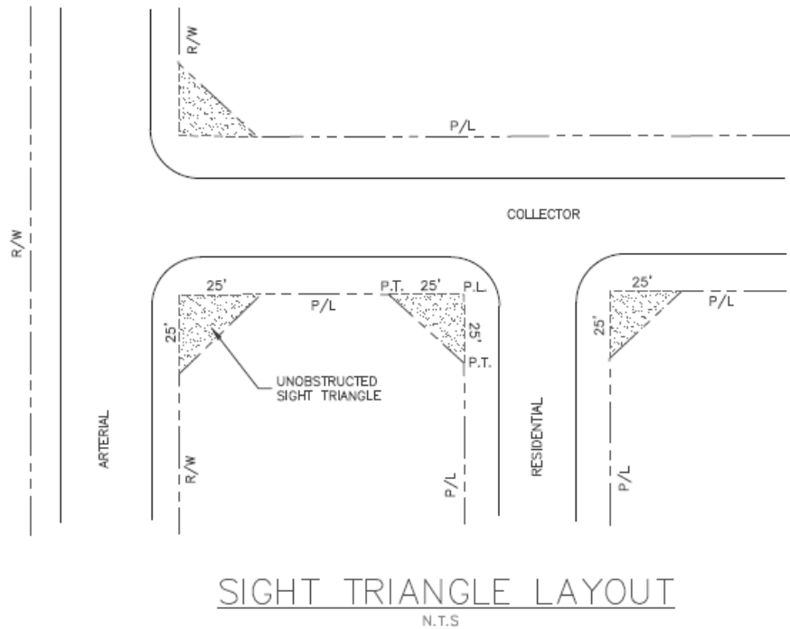
Exhibit 8.4 Sight Triangles
