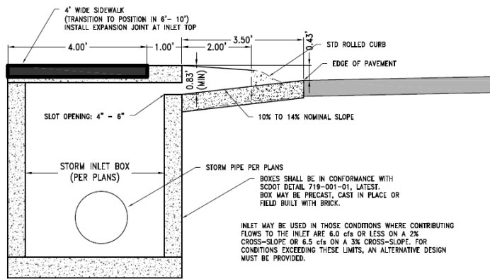
TYPE 9 INLET (RUN LOCATION) NOT TO SCALE
